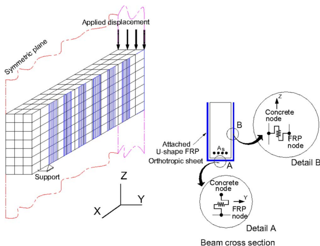
Fig. 3. Finite-element model
