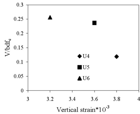
Fig. 13. Comparison between the shear capacity ( V/bdf_c ) against the vertical strain at middepth of Strip F3 for the U-wrap strengthened specimens
