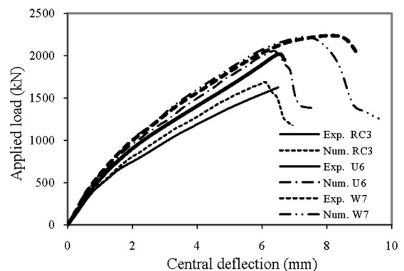
Fig. 8. Load-deflection relationships for the specimens of the third set
