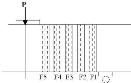
Fig. 2. Strip notations along the shear span
