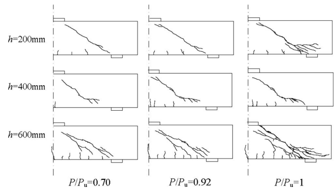
Fig. 4. Crack patterns of the control specimens at various load levels
