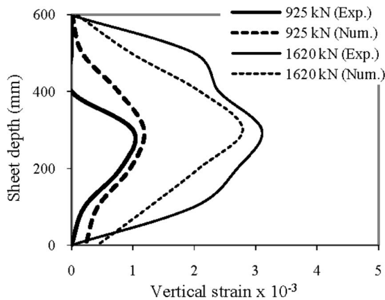
Fig. 11. Axial strain profiles along the CFRP depth for F3 bonded strip of Specimen U6
