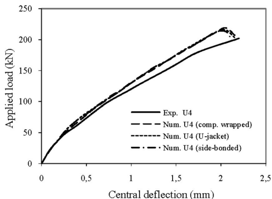
Fig. 6. Comparison of load-deflection relationships for Specimen U4 with various strengthening configurations
