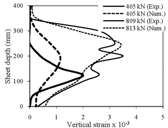
Fig. 10. Axial strain profiles along the CFRP depth for F3 bonded strip of Specimen U5
