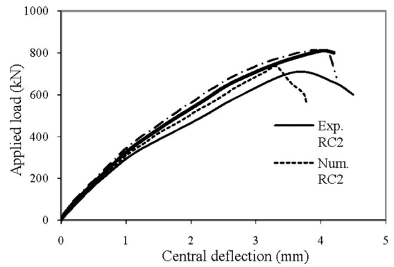
Fig. 7. Load-deflection relationships for the specimens of the second set
