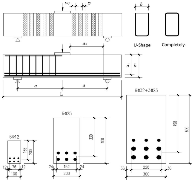
Fig. 1. Specimen configuration details
