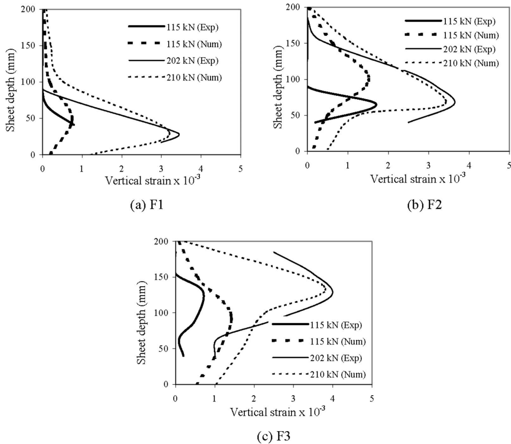
Fig. 9. Axial strain profiles along the CFRP depth for F1, F2, and F3 bonded strips of Specimen U4
