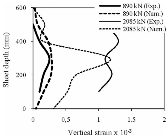
Fig. 12. Axial strain profiles along the CFRP depth for F3 bonded strip of Specimen W7
