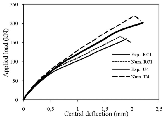
Fig. 5. Load-deflection relationships for the specimens of the first set
