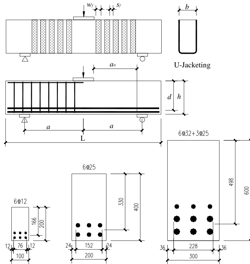
Figure 2 Configurations of specimens
