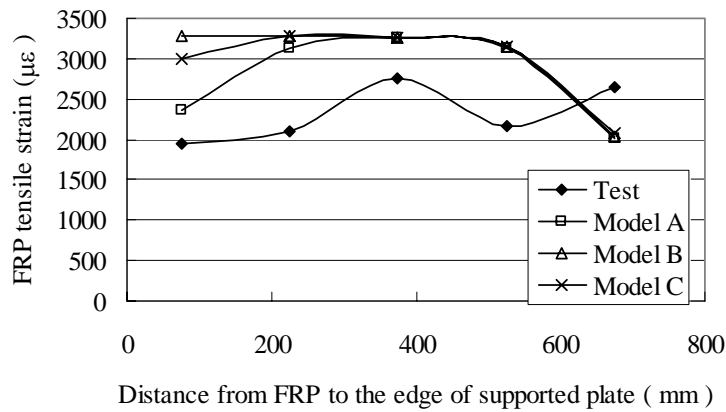
Figure 7 FRP strain distribution for different diagonal crack models: specimen U6
