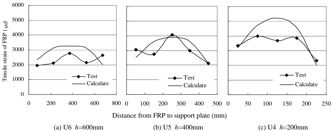
Figure 8 Measured FRP strain distribution along the diagonal crack versus FE prediction
