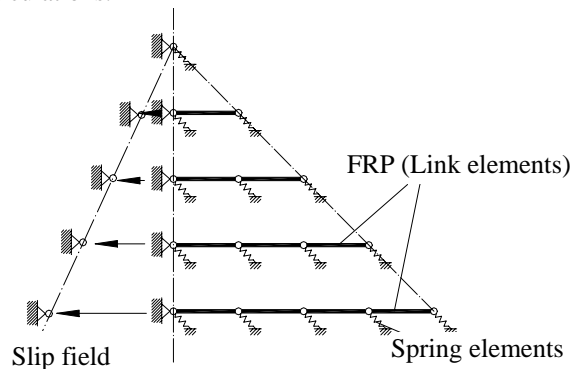
Figure 5 Simplified FE model for externally bonded FRP U-jackets on RC beam
