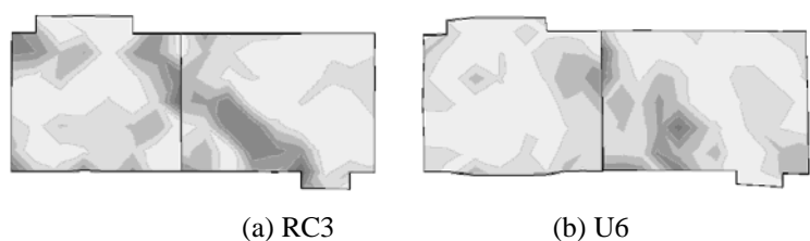
Figure 11 Principle tensile strain distributions on the webs of RC3 and U6 at a load of P \approx 0.75/P_u
