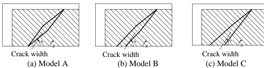
Figure 6 Simplified diagonal crack models by Lu et al. (2005a)
