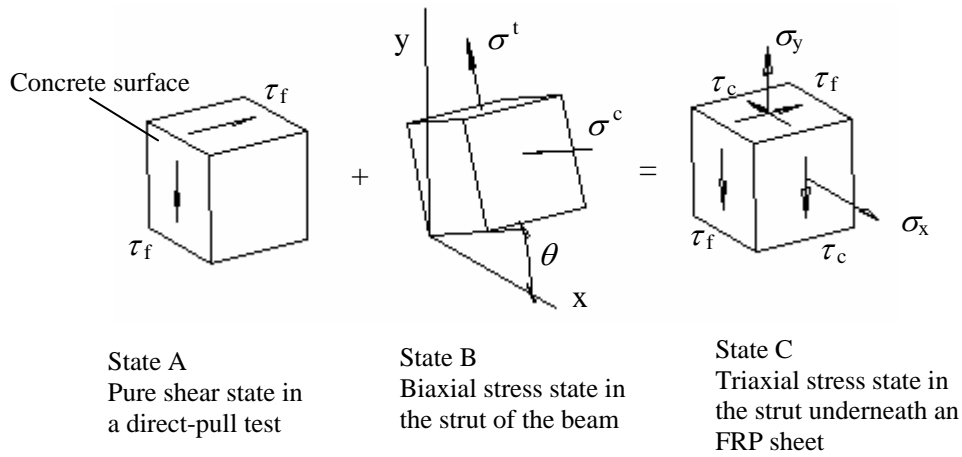
Figure 4 Superposition of stress states of concrete in the strut underneath the FRP sheets
