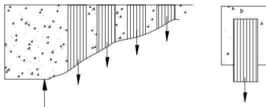
(a) FRP externally bonded on the web in shear (b) Direct-pull test
